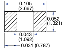
0705 Land Pattern
